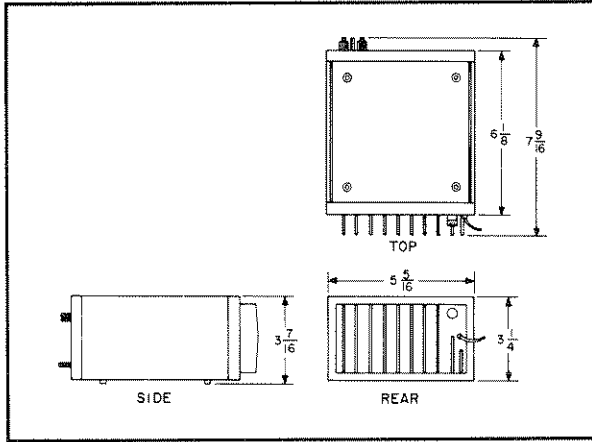
Figure 2-1. Outline Diagram
